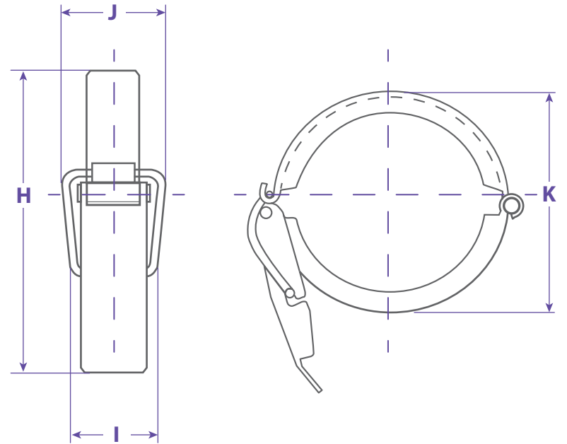
Locking Ring
